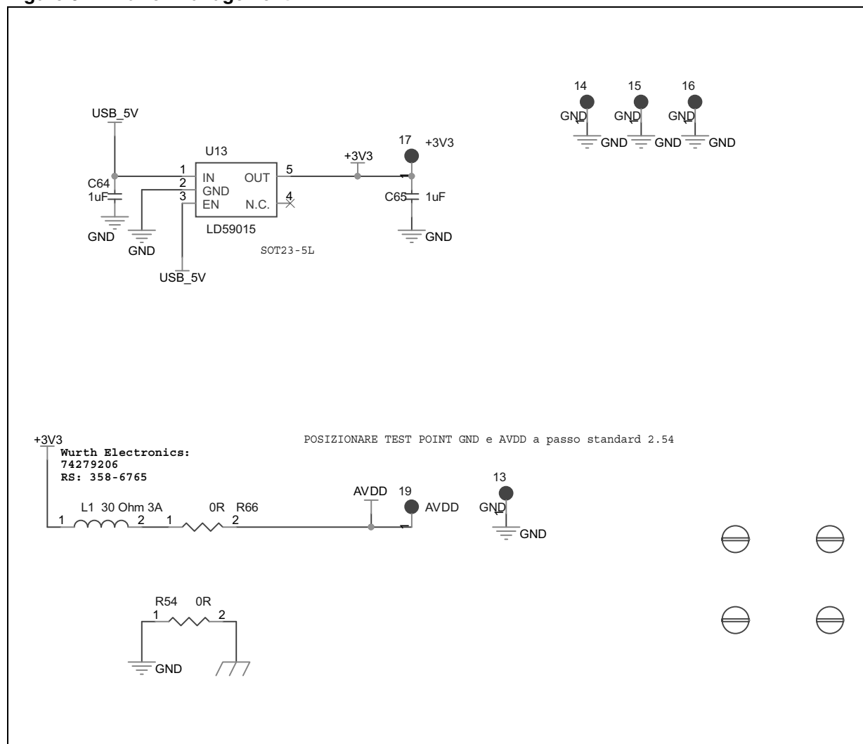
Figure 6. Power management
